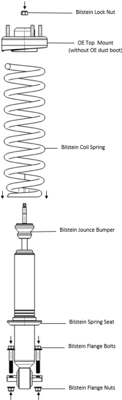
Figure 4: Assembly
