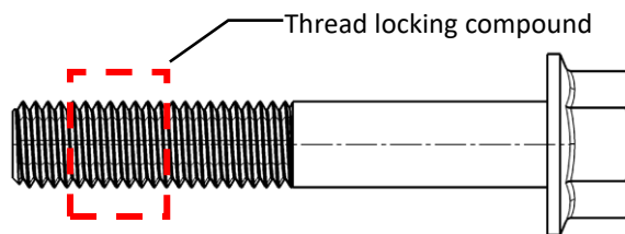
Figure 3: Supplied Flange Bolt
