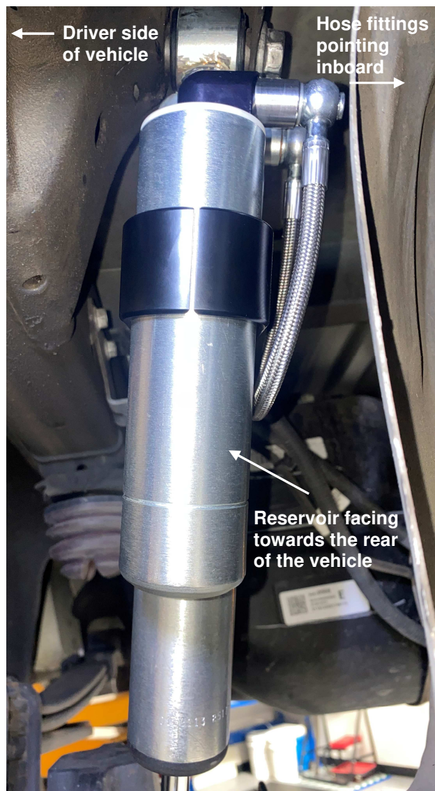
Figure 5. Driver Side (Rear View)
