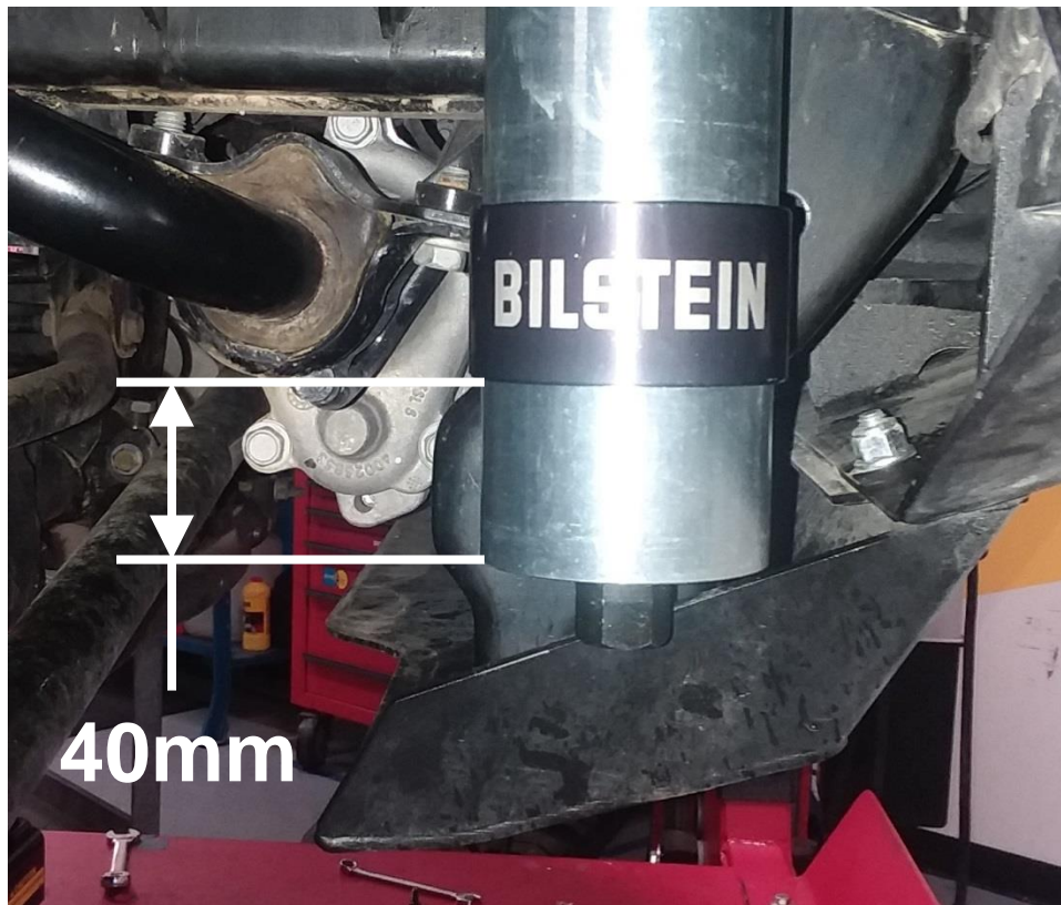
Figure 26 – Reservoir Height
