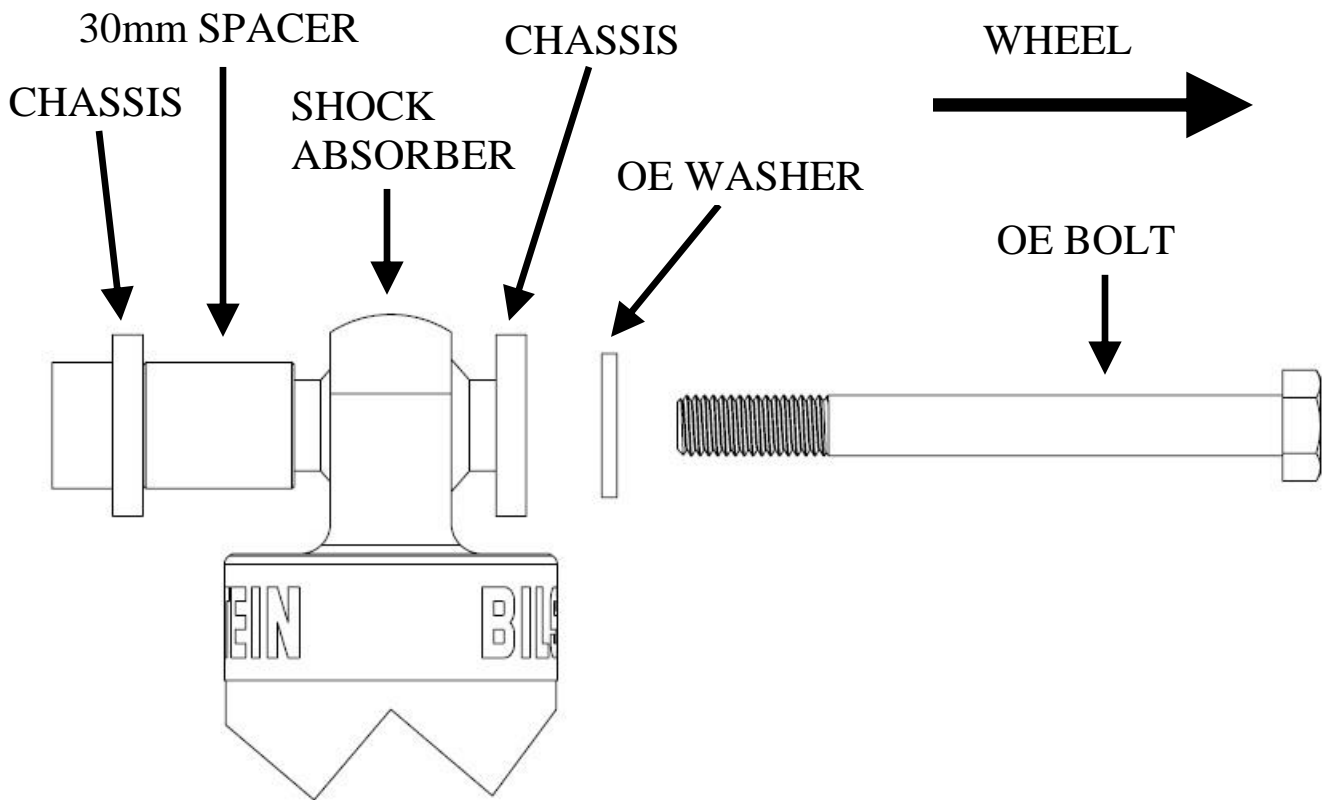
Figure 17 – Vehicle Right Side Upper Mount Assembly Diagram
