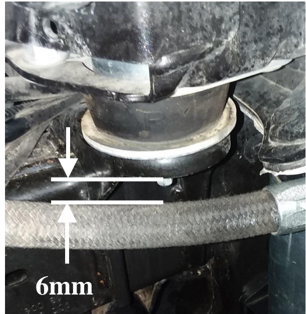
Figure 33 – Right Side Reservoir Hose Clearance
