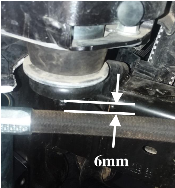
Figure 32 – Left Side Reservoir Hose Clearance
