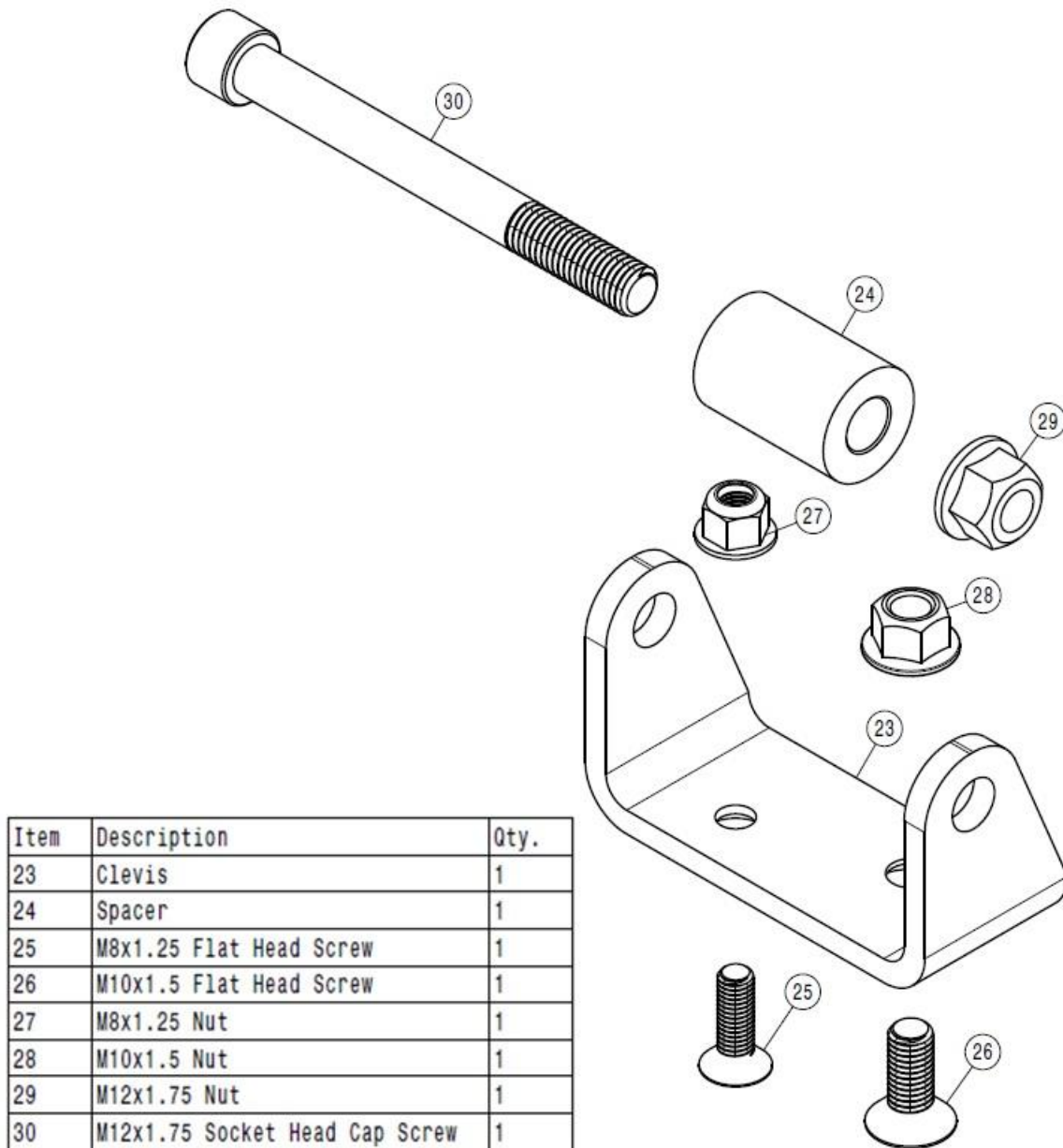
Figure 19 – Lower Mount Offset Bracket
