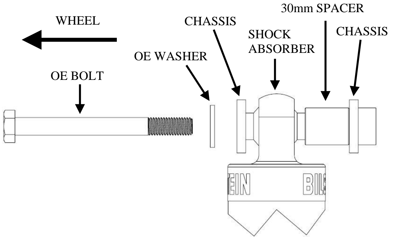
Figure 15 – Vehicle Left Side Upper Mount Assembly Diagram
