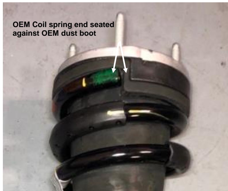
Figure 4: OEM Coil spring clocking
